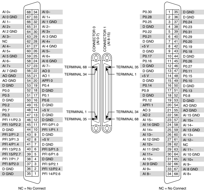
Figure 6. NI PXIe-6358 Pinout
